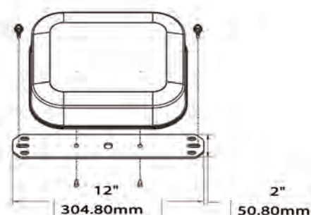
Mounting Bracket Flat/Blind for Eclipse Series
