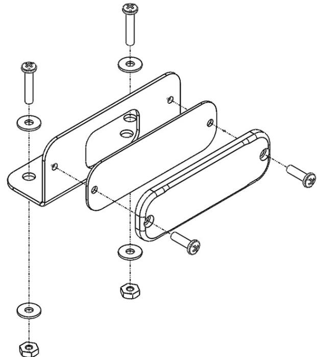
6" OVAL BRACKET KIT 98601
