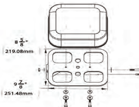
Bracket Side Mounting for Eclipse Series Mini Lightbar
