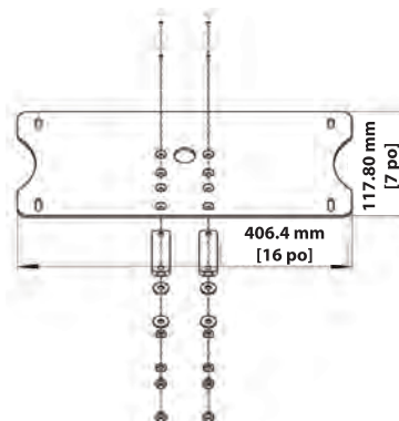
Bracket Kit 16" Minibar Mounting Plate
