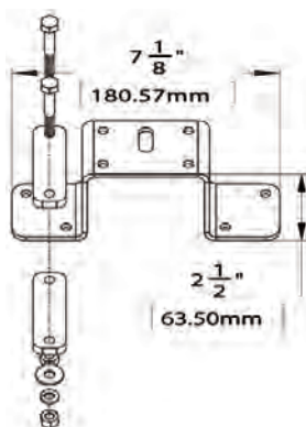
Bracket Kit 2.5" Riser Kit for 98012
