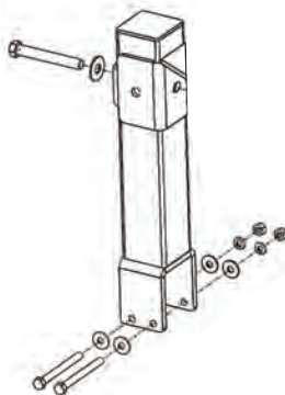
10" EXTENSION BRACKET KIT 98043
